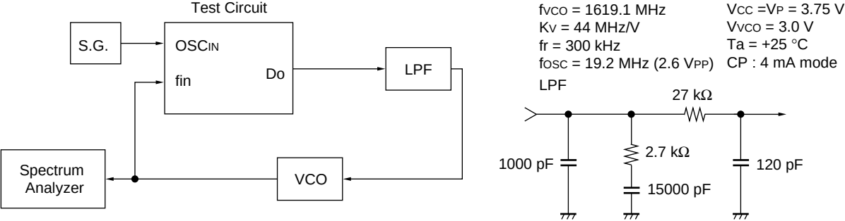
PLL Reference Leakage
