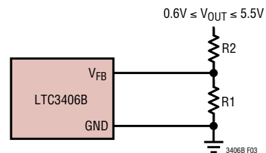
Figure 3. Setting the LTC3406B Output Voltage
