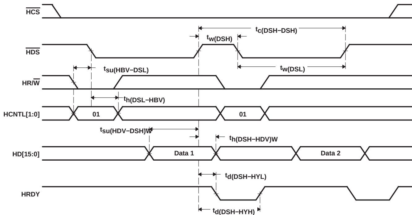
Figure 5-30. Multiplexed Write Timings With \overline{\text{HCS}} Held High
