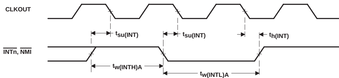
Figure 5-13. Interrupt Timing
