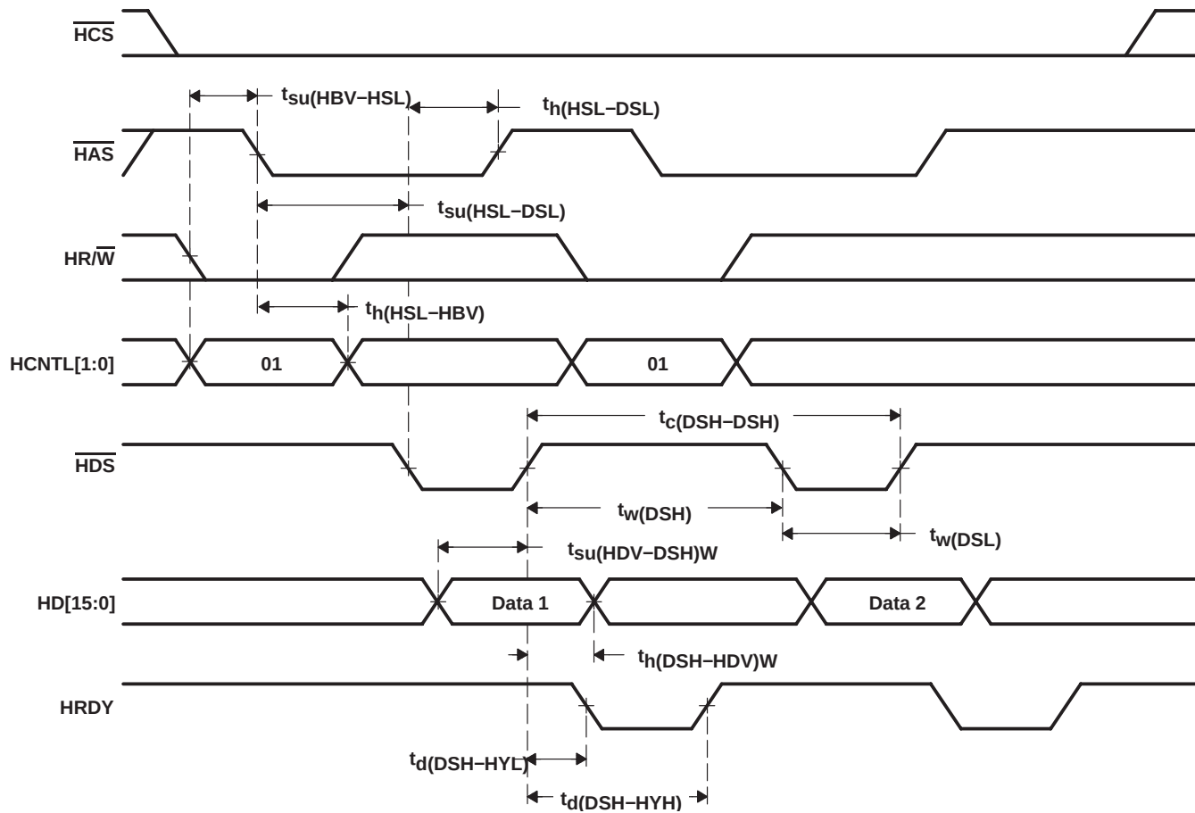
Figure 5-29. Multiplexed Write Timings Using \overline{HAS}
