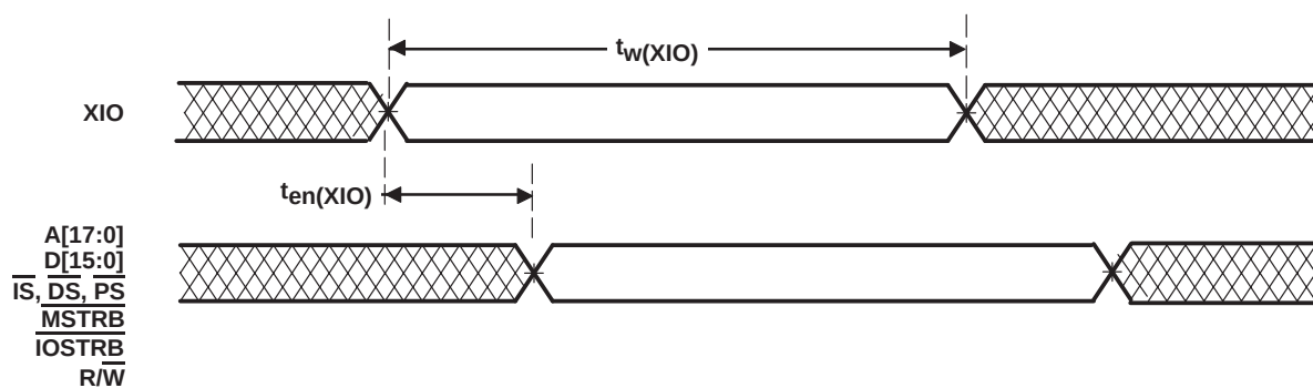
Figure 5-14. XIO Timing
