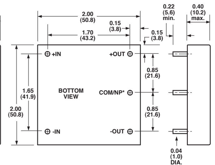
ALTERNATIVE PIN CONFIGURATION SUFFIX "S"
