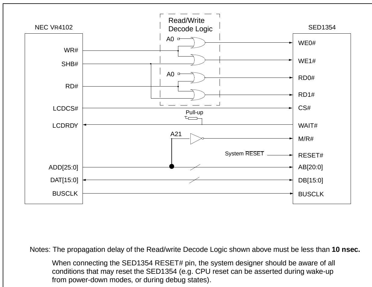
Figure 4-1: Typical Implementation of VR4102 to SED1354 Interface
