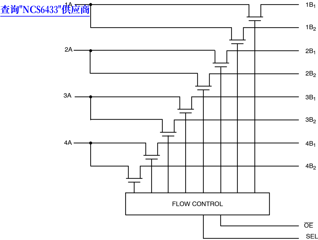
Figure 1. NCS6433 Block Diagram
