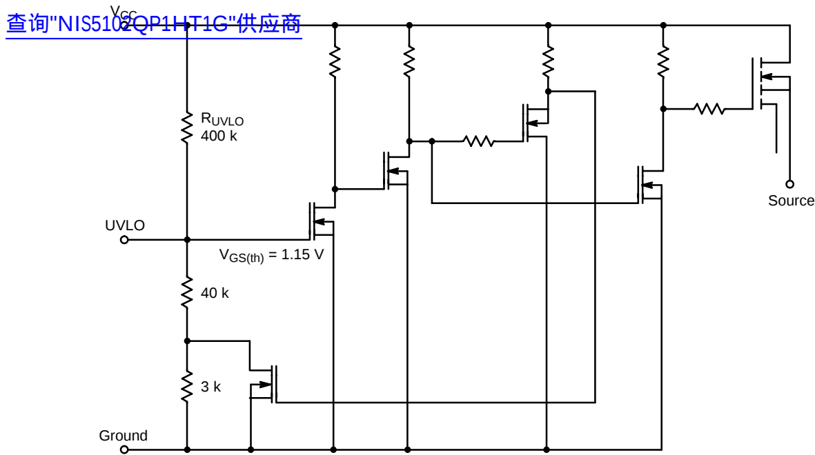
Figure 18. Equivalent Undervoltage Lockout Circuit
