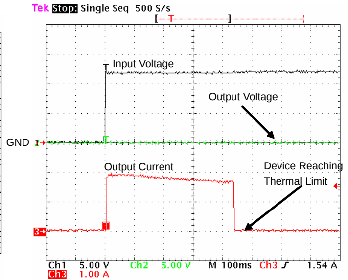
Figure 11. Turn-on Waveforms for Shorted Output, Latchoff Device
