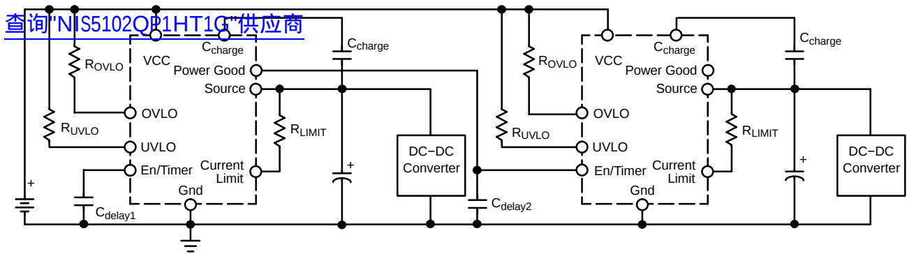
Figure 14. Turn-on Sequencing Using Power Good Signal
