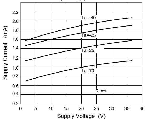
Fig.1 Supply Current
