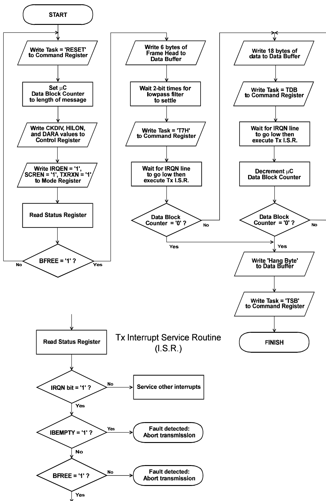
Figure 14 Transmit Process
