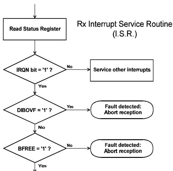
Figure 15 Receive Process
