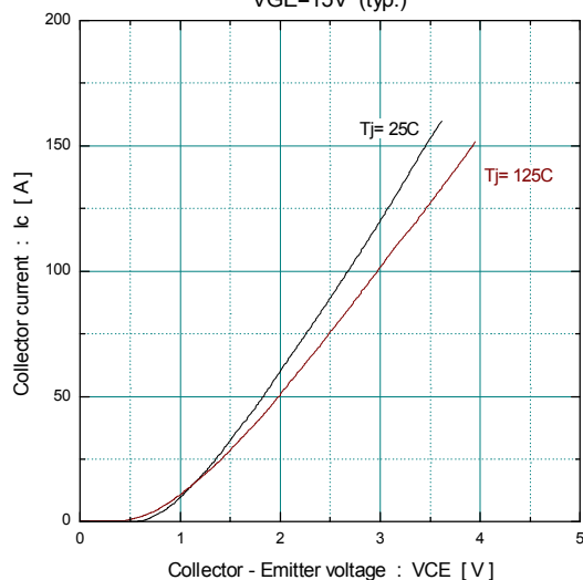
③ Collector current vs. Collector-Emitter voltage VGE=15V (typ.)
