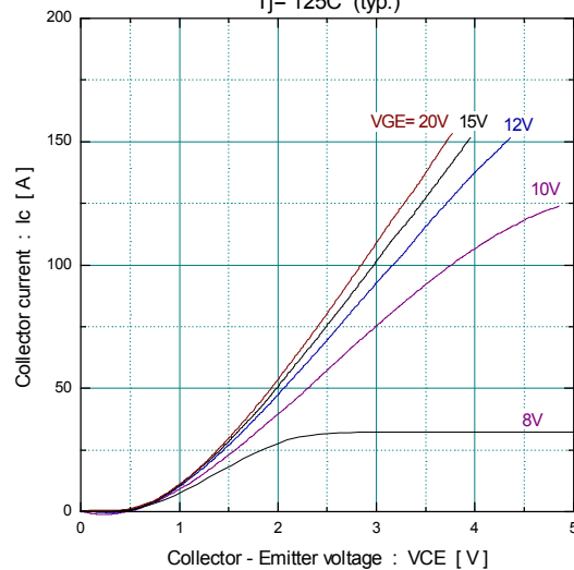
② Collector current vs. Collector-Emitter voltage Tj= 125C (typ.)
