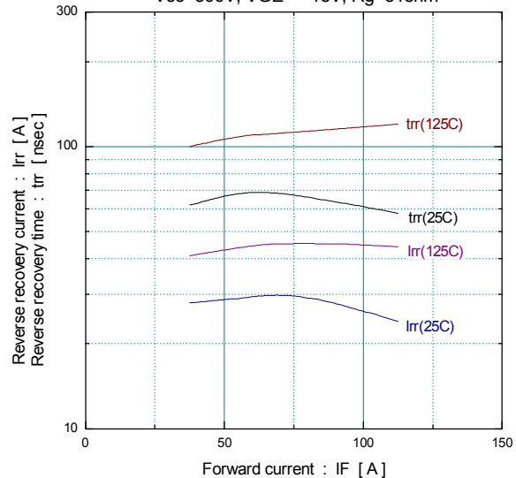
Reverse recovery characteristics (typ.) Vcc=300V, VGE=+-15V, Rg=51ohm
