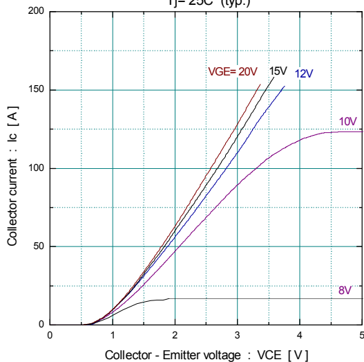
① Collector current vs. Collector-Emitter voltage Tj= 25C (typ.)
