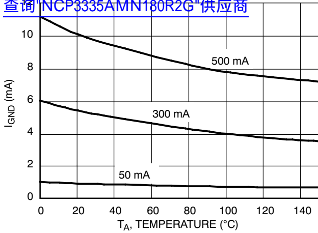
Figure 17. Ground Current vs. Temperature
