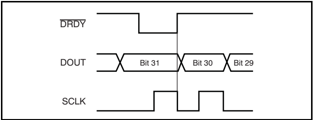
Figure 60. DRDY with Data Retrieval
