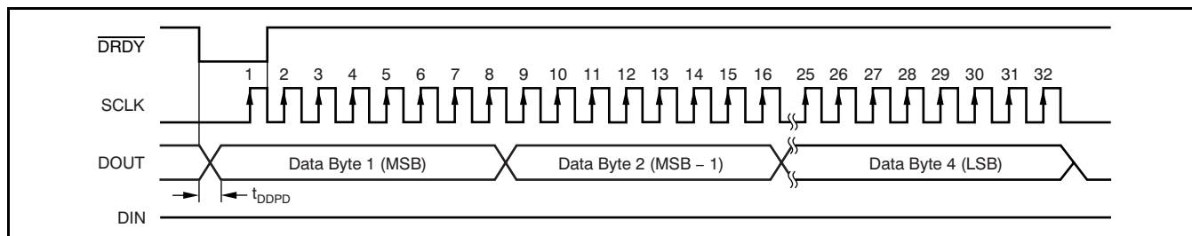
Figure 62. Read Data Continuous
