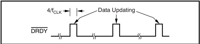
Figure 61. DRDY With No Data Retrieval
