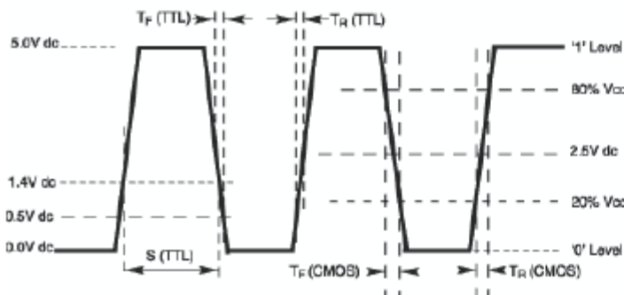
OUTPUT WAVEFORM
