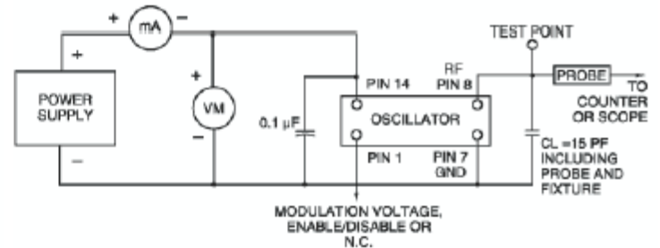
TEST CIRCUIT DIAGRAM
