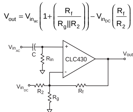
Fig. 4 Level Shifting Circuit
