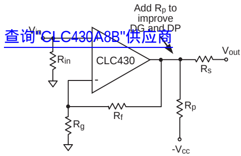
Fig. 3 Improved DG and DP Video Amplifier
