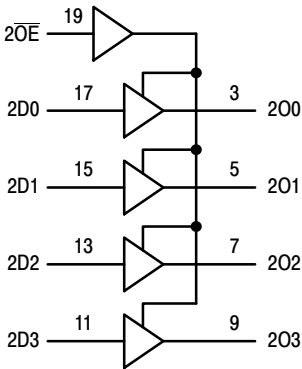
Figure 2. Logic Diagram
