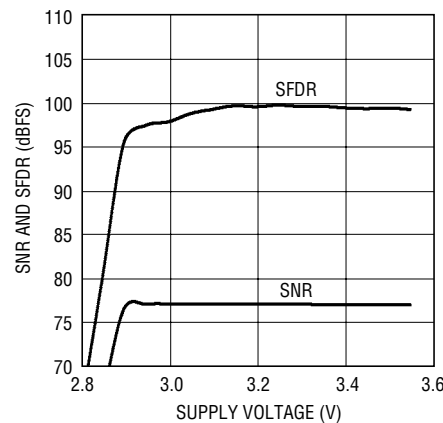
SNR and SFDR vs Supply Voltage ( V_{DD} ), f_{IN} = 5.1\text{MHz} , -1\text{dBFS}
