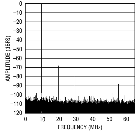
32k Point FFT, f_{IN} = 380.11\text{MHz} , -1\text{dBFS} , PGA = 1, RAND = “On”, Dither “Off”
