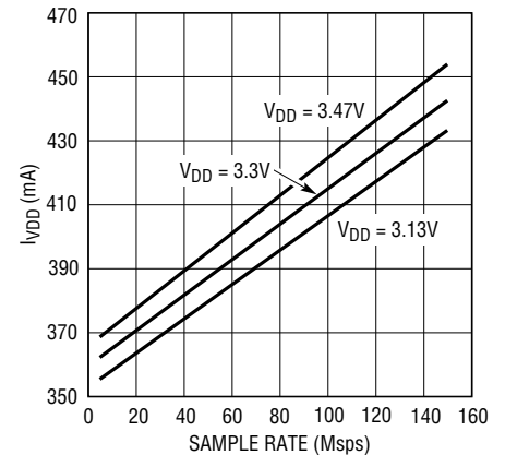
I_{VDD} vs Sample Rate, f_{IN} = 5.1\text{MHz} , -1\text{dBFS}
