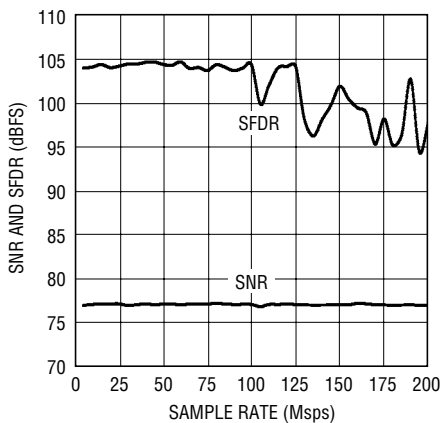
SNR and SFDR vs Sample Rate f_{IN} = 5.1\text{MHz} , -1\text{dBFS}
