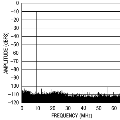
32k Point FFT, f_{IN} = 250.11\text{MHz} , -10\text{dBFS} , PGA = 1, RAND = “On”, Dither “Off”
