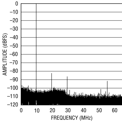
32k Point FFT, f_{IN} = 250.11\text{MHz} , -1\text{dBFS} , PGA = 1, RAND = “On”, Dither “Off”
