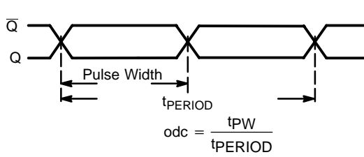
Figure 6. Output Duty Cycle/Pulse Width/Period
