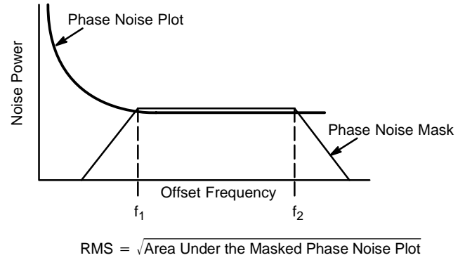
Figure 5. RMS Phase Jitter
