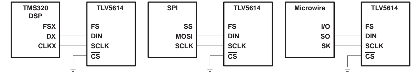
Figure 17. Three-Wire Interface
