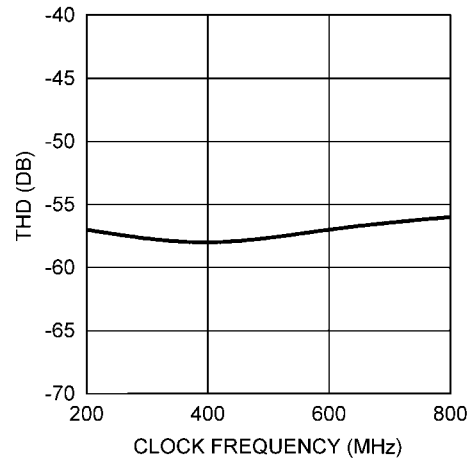
THD vs. SAMPLE RATE
