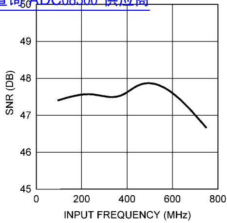
查询"ADC08500"供应商 SNR vs. INPUT FREQUENCY
