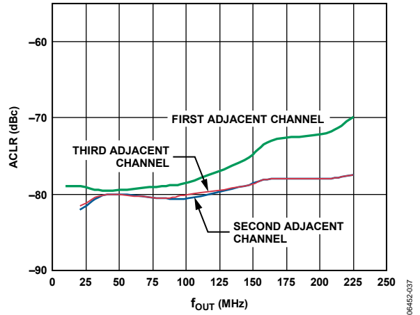
Figure 40. AD9778A ACLR, Single Carrier W-CDMA, 4\times Interpolation, f_{DATA} = 122.88 MSPS, Amplitude = -3 dBFS
