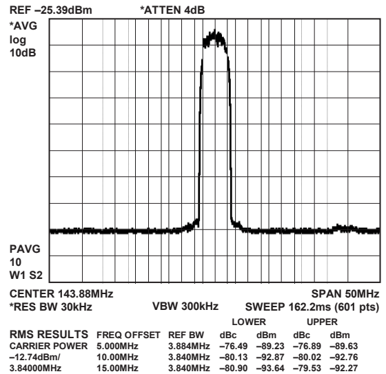
Figure 41. AD9778A ACLR, f_{DATA} = 122.88 MSPS, 4\times Interpolation, f_{DAC}/4 Modulation
