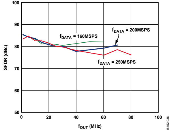
Figure 39. AD9778A In-Band SFDR vs. f_{OUT} , 2\times Interpolation
