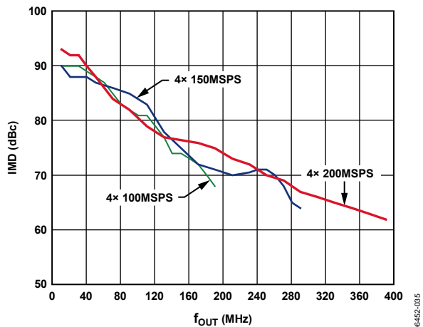
Figure 38. AD9778A IMD vs. f_{OUT} , 4\times Interpolation
