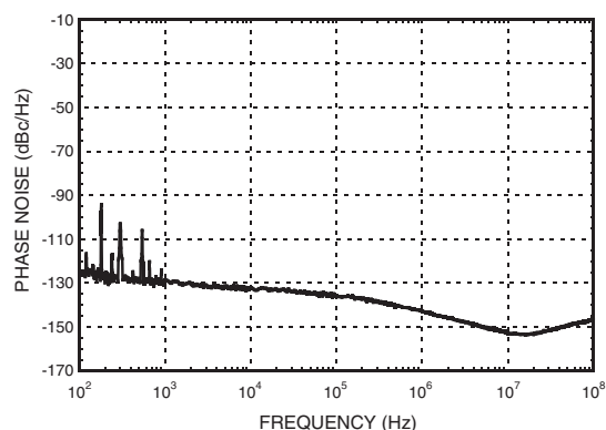
Phase Noise @ 19 GHz
