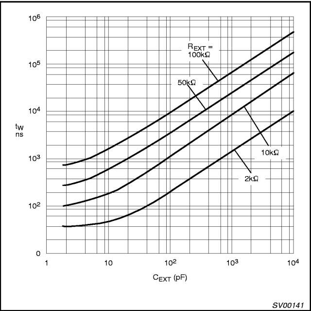
Figure 5. Typical output pulse width as a function of the external capacitor values at V CC = 3.3V and T amb = 25°C.
