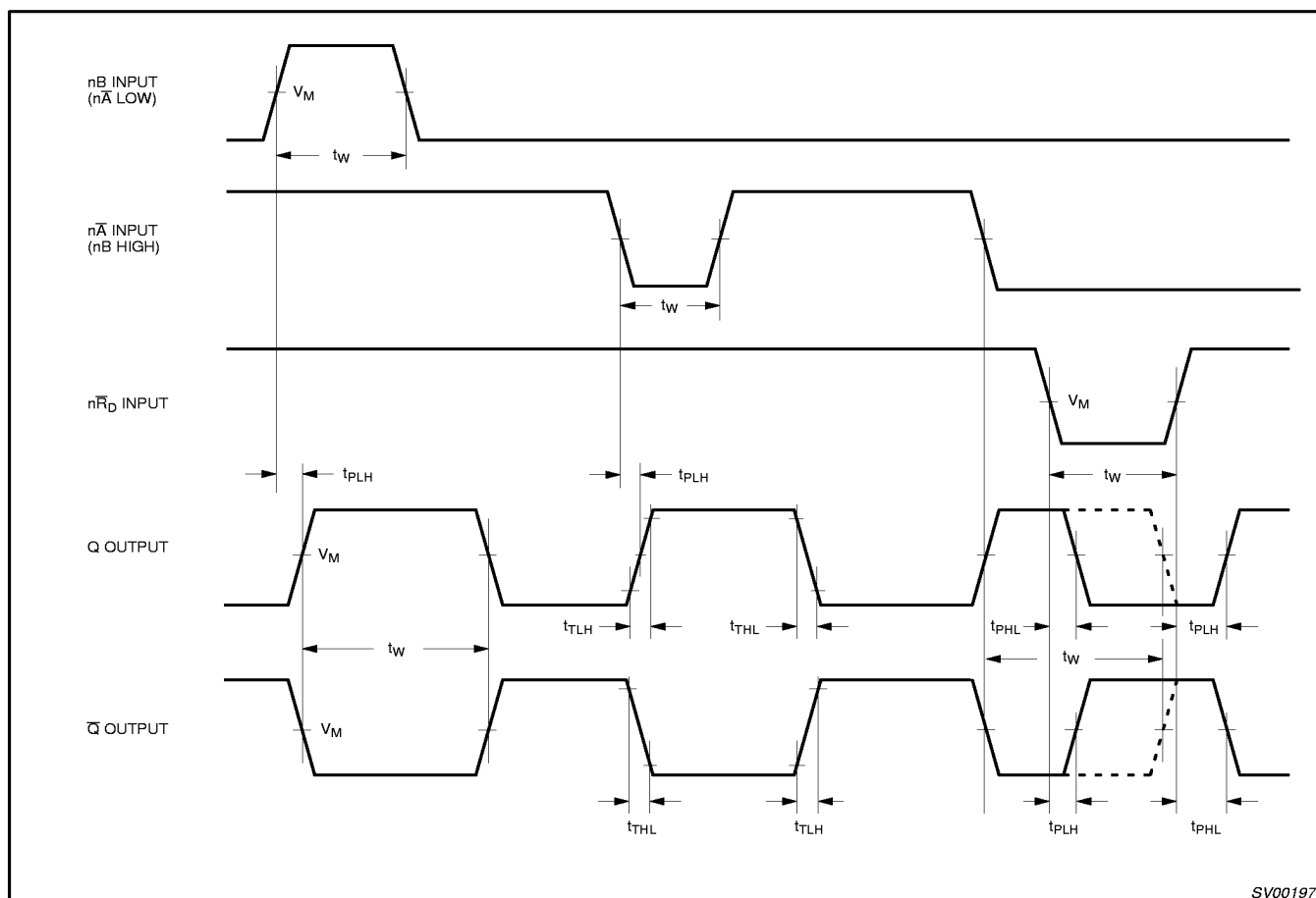
Figure 3. Input ( nA , nB , nRD ) to output ( nQ , n\bar{Q} ) propagation delays, the output transition times, and the input and output pulse widths.
