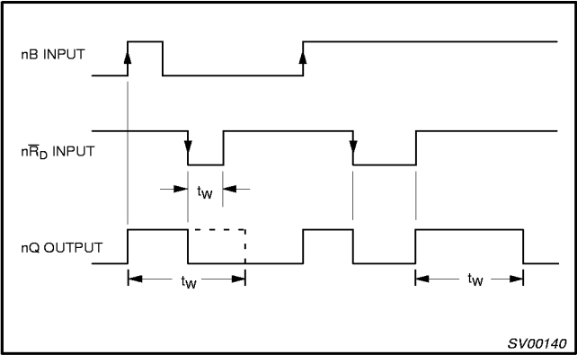
Figure 2.Output pulse control using reset input n\overline{R}_D ; n\overline{A} = \text{LOW} .
