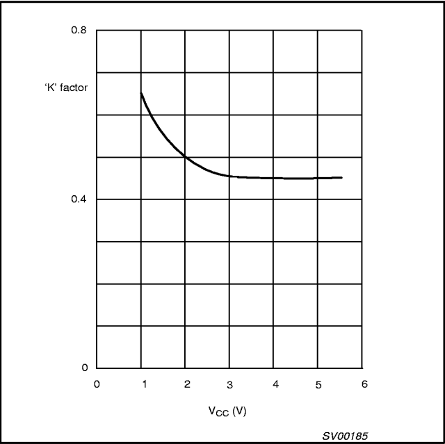
Figure 4. HCT typical "k" factor as a function of V CC ; C X = 10 nF; R X = 10 K \Omega to 100 K \Omega .
