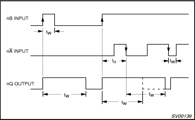
Figure 1.Output pulse control using retrigger pulse; n\overline{R}_D = \text{HIGH} .
