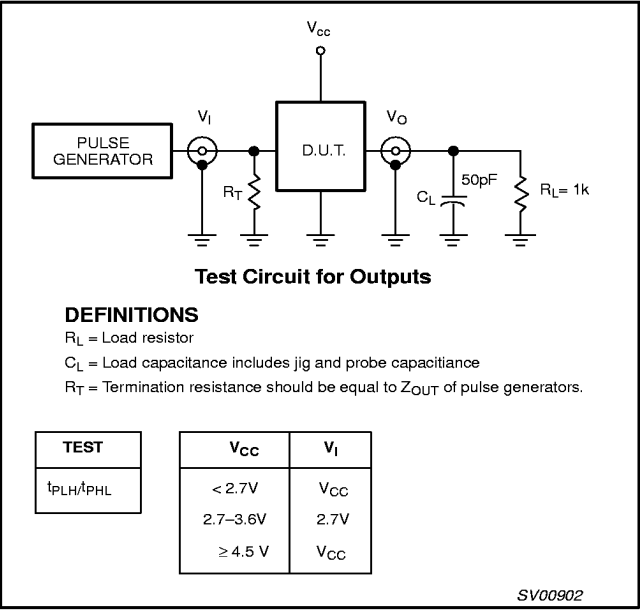
Figure 8. Load circuitry for switching times
