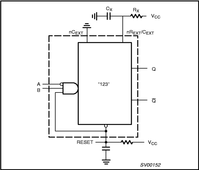
Figure 6. Power-up output pulse elimination circuit
