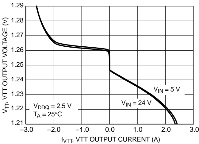
Figure 11. VTT Output Voltage (DDR) vs. VTT Output Current
