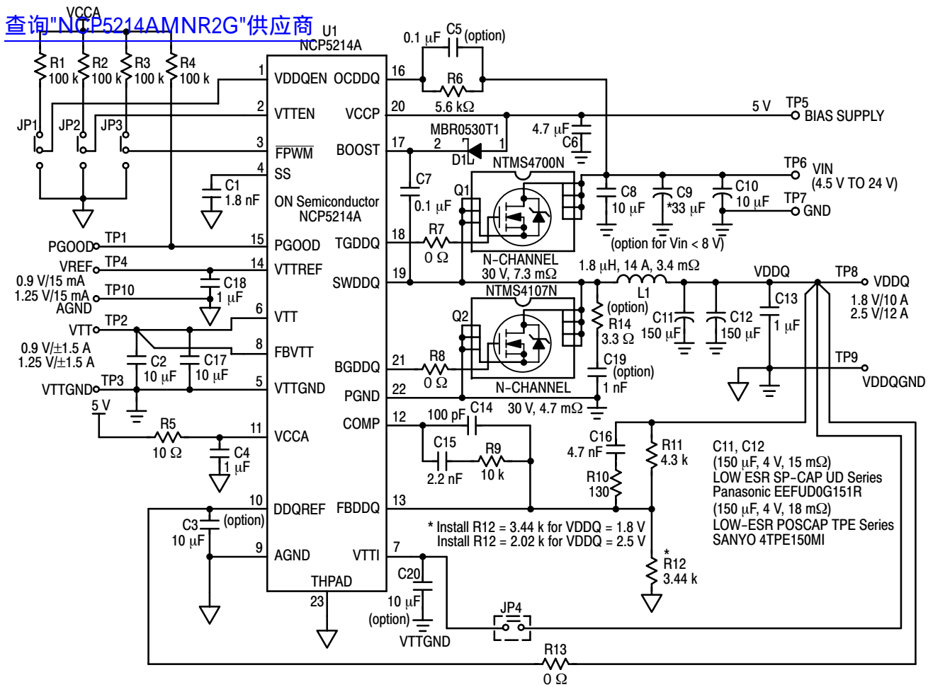
Figure 41. Schematic Diagram of Evaluation Board
