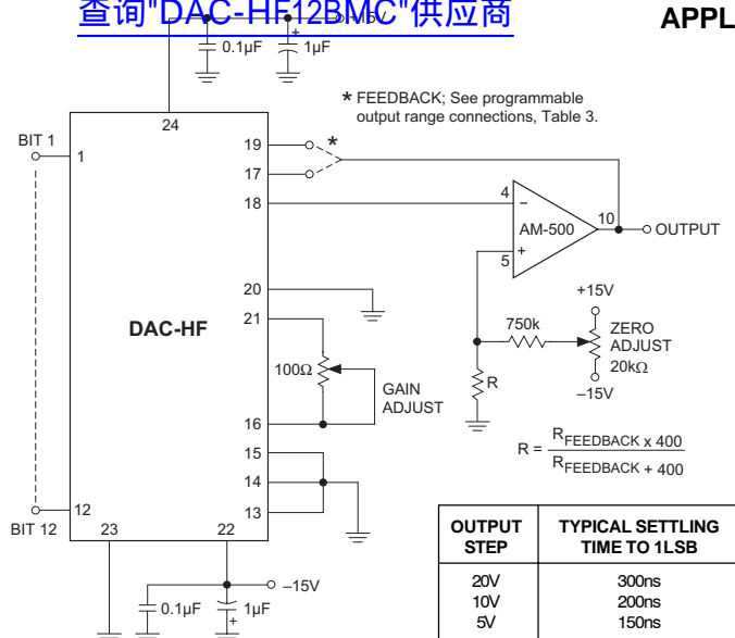
Figure 6. Unipolar Ultra-Fast Voltage Output Circuit
