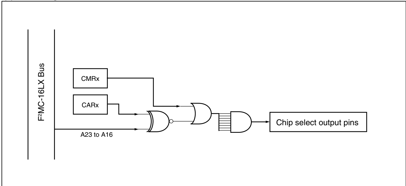
(2) Block Diagram
