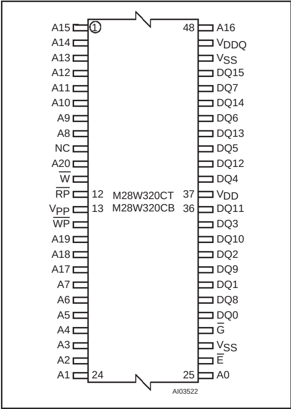
Figure 3. TSOP Connections
