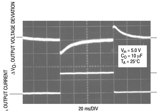
Figure 2. Transient Load Regulation
