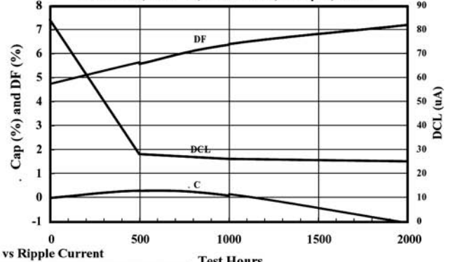
Life Test, 105 °C, Full Load, 330 \mu\text{F} , 400 V
