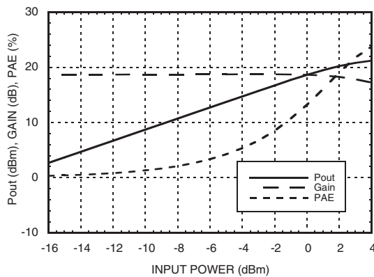
Power Compression @ 2100 MHz [1]
