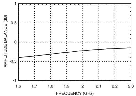
Magnitude Balance [1]
