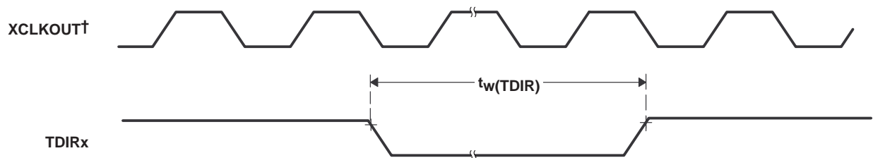
Figure 6–16. TDIRx Timing
