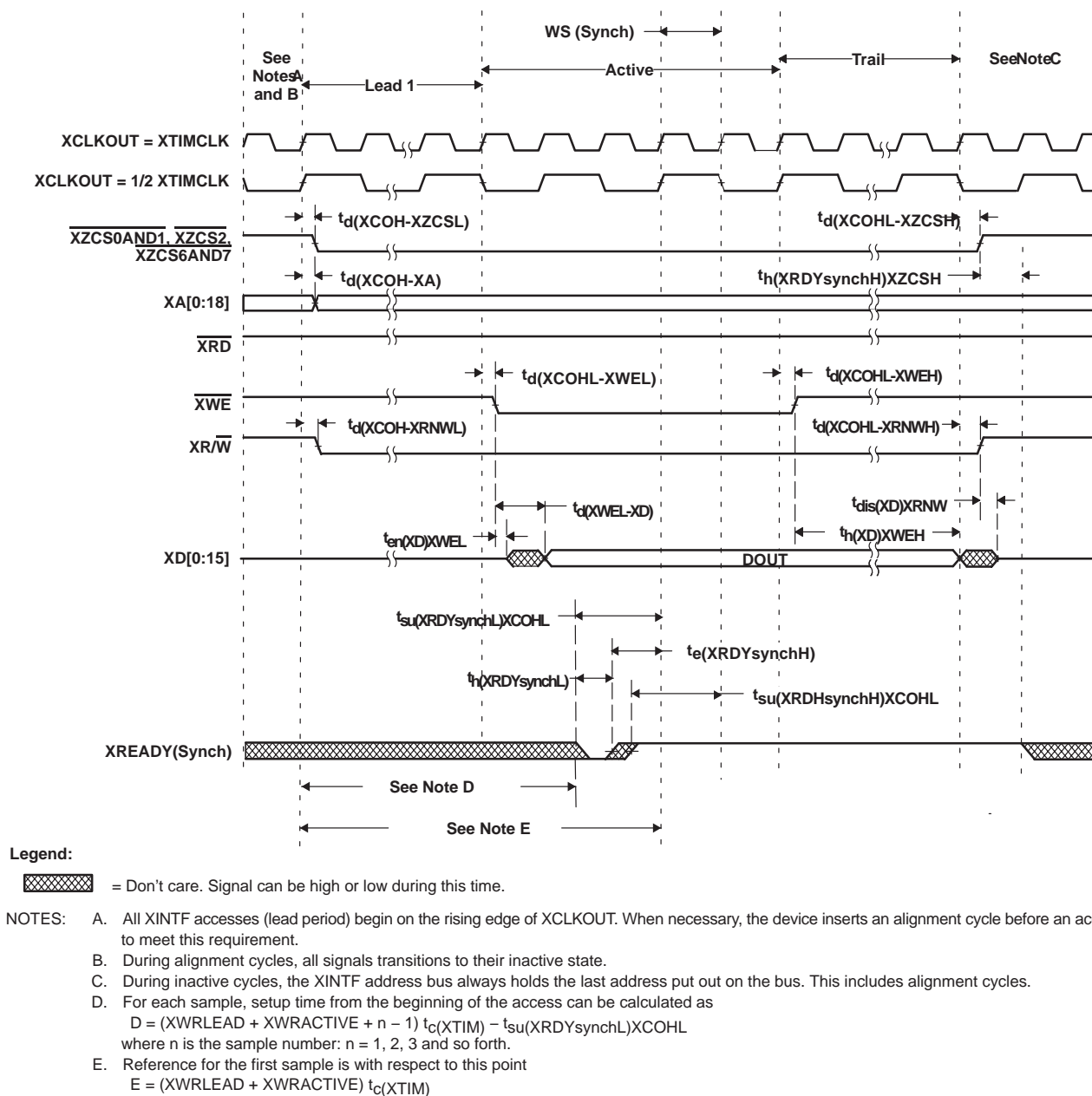
Figure 6–32. Write With Synchronous XREADY Access
