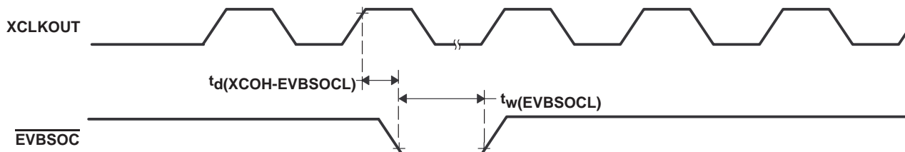
Figure 6–18. EVBSOC Timing
