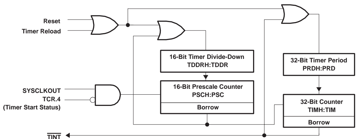
Figure 4–1. CPU-Timers
