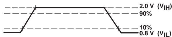
Figure 6–5. Input Levels
