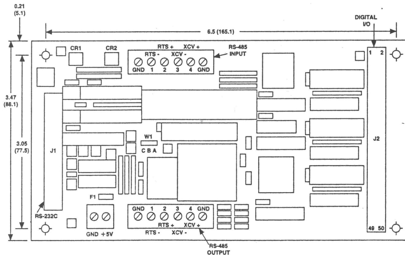
Figure 5. Outline Dimensions
