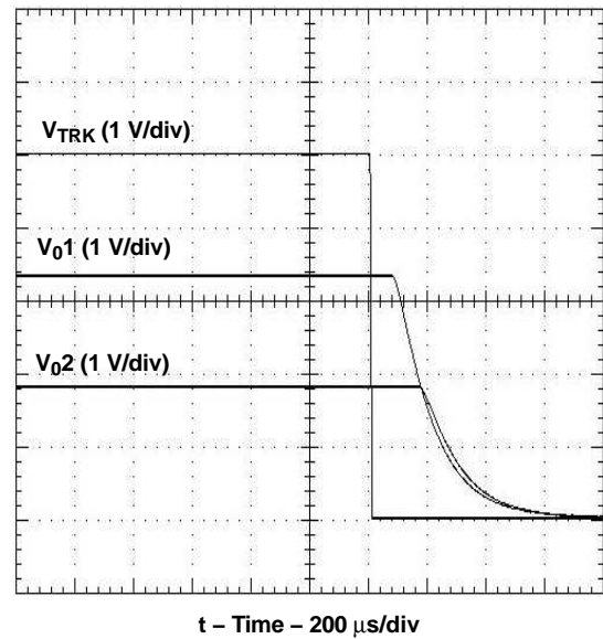
Figure 17. Auto-Track Simultaneous Power Down Waveforms
