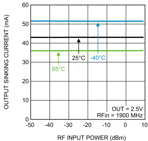
Output Sinking Current vs. RF Input Power
