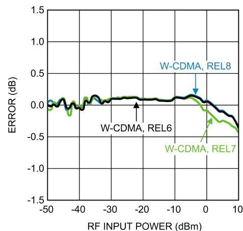
FIGURE 13. Variation due to Modulation for W-CDMA at 1900 MHz
