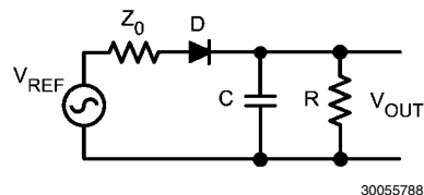
FIGURE 3. Diode Detector
