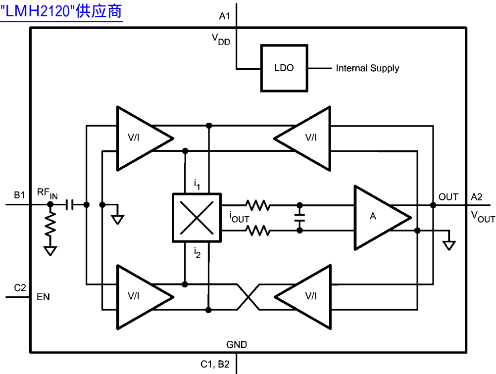
FIGURE 4. Block Diagram
