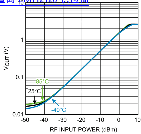
Output Voltage vs. RF Input Power at 900 MHz 查询"LMH2120"供应商
