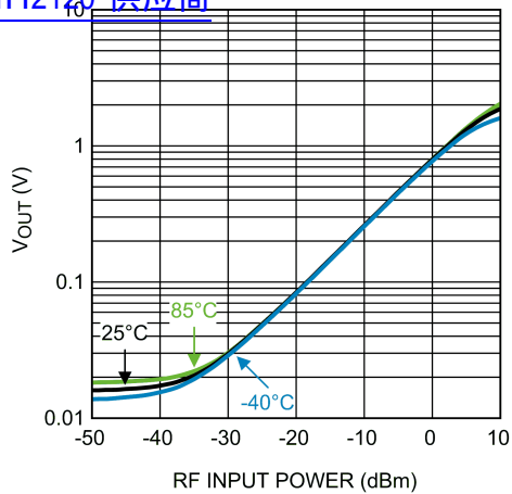
Output Voltage vs. RF Input Power at 2600 MHz 查询"LMH2120"供应商
