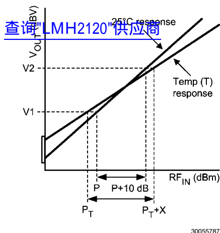
FIGURE 11. Graphical Representation of 10 dB Step Error Calculations
