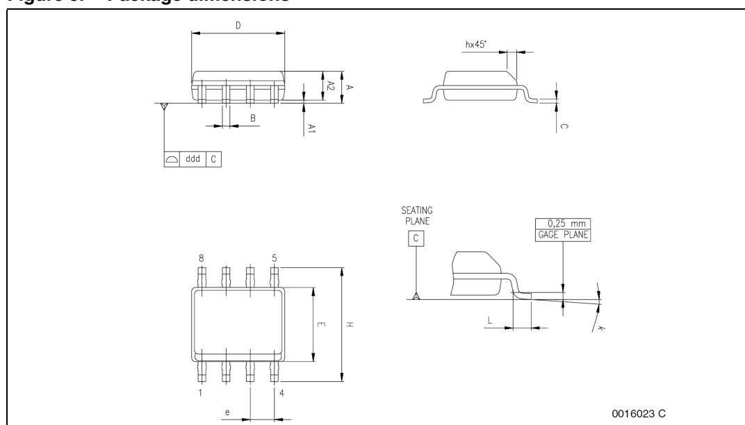
Figure 9. Package dimensions
