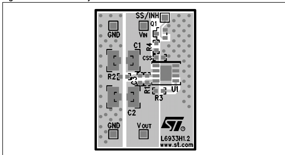
Figure 7. Demoboard layout
