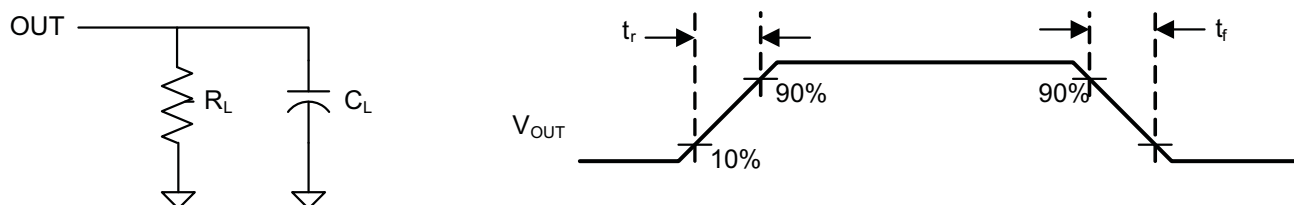
TEST CIRCUIT
