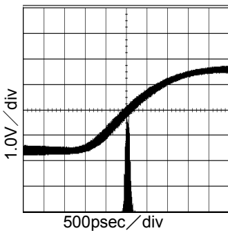
Fig.13 24.576MHz Period-Jitter VDD=3.3V,CL=15pF
