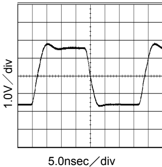
Fig.18 BUF_OUT(27MHz) output waveform VDD=3.3V,CL=50pF
