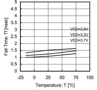
Fig.49 54MHz Temperature - fall-time
