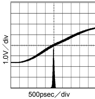
Fig.19 BUF_OUT(27MHz) Period-Jitter VDD=3.3V,CL=50pF
