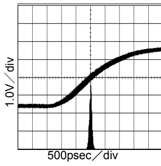
Fig.4 33.8688MHz Period-Jitter VDD=3.3V,CL=32pF
