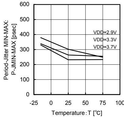
Fig.51 54MHz Temperature - Period-Jitter MIN-MAX
