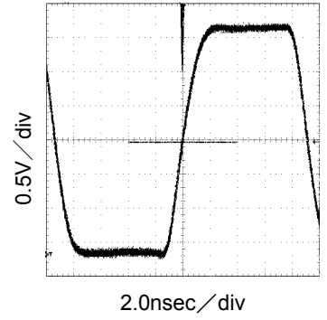
Fig.69 54MHz Long Term Jitter
