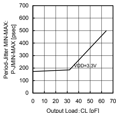
Fig.71 36.864MHz CL – Period-Jitter MIN-MAX
