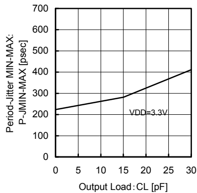
Fig.73 24.576MHz CL – Period-Jitter MIN-MAX
