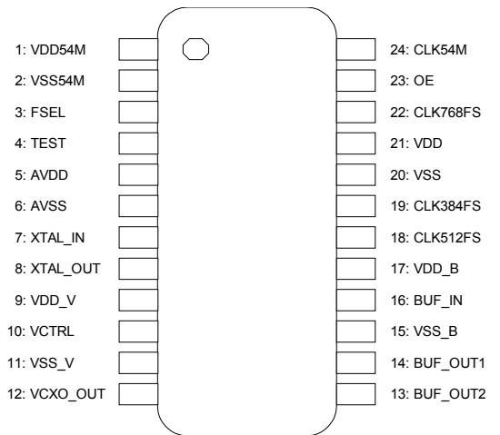
Fig.78 Pin assignment
