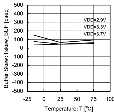
Fig.56 27MHz BUFFER Temperature - Skew (BUF_OUT2 Phase Lead)
