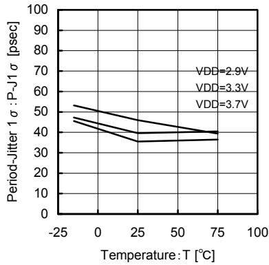
Fig.50 54MHz Temperature - Period-Jitter 1 sigma
