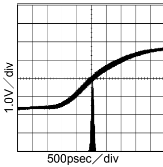
Fig.10 18.432MHz Period-Jitter VDD=3.3V,CL=32pF
