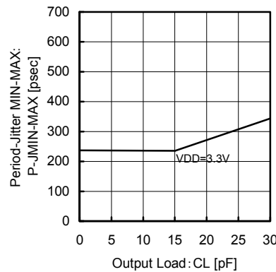
Fig.74 54MHz CL – Period-Jitter MIN-MAX
