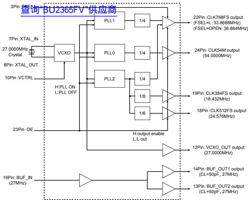
Fig.77 Block diagram
