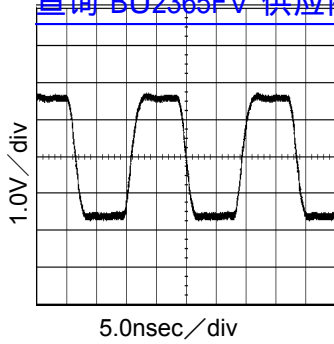
Fig.15 54MHz output waveform VDD=3.3V,CL=15pF
