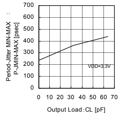
Fig.72 18.432MHz CL – Period-Jitter MIN-MAX
