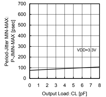
Fig.75 27MHz VCXO CL – Period-Jitter MIN-MAX
