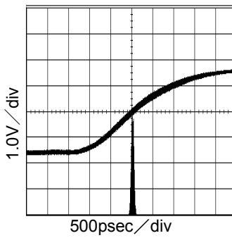
Fig.7 36.864MHz Period-Jitter VDD=3.3V,CL=32pF
