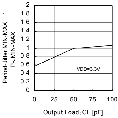
Fig.76 27MHz BUFFER CL – Period-Jitter MIN-MAX
