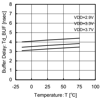
Fig.55 27MHz BUFFER Temperature - Delay
