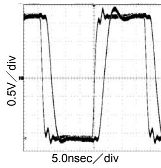
Fig.25 Buffer delay(IN→OUT1) VDD=3.3V,CL=50pF
