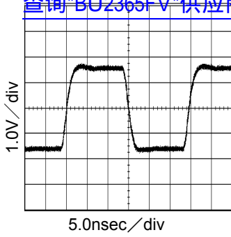
Fig.3 33.8688MHz output waveform VDD=3.3V,CL=32pF
