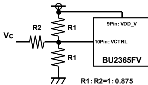
Fig.1 Control Circuit of Control Voltage
