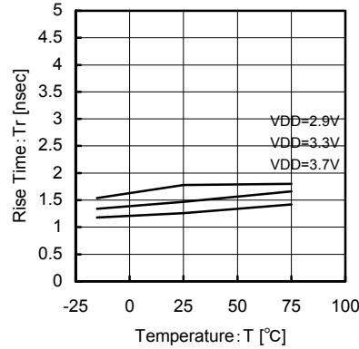
Fig.48 54MHz Temperature - rise-time
