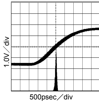
Fig.16 54MHz Period-Jitter VDD=3.3V,CL=15pF
