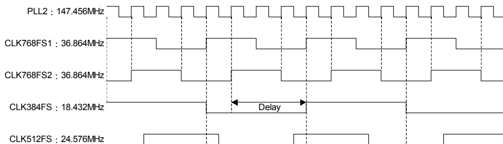
Fig.79 Audio Clock Output Circuit Configuration and Timing Chart
