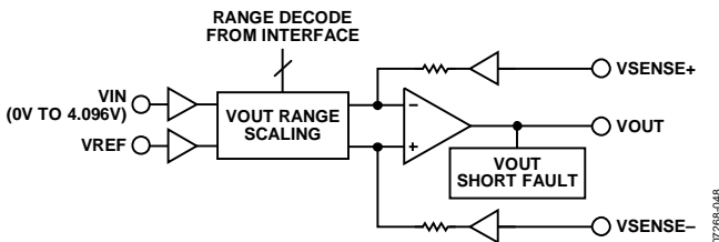
Figure 54. Voltage Output
