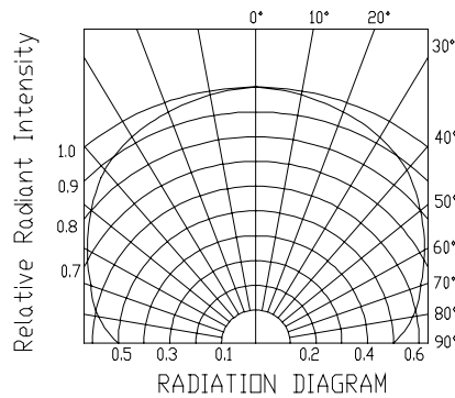
Radiation Diagram T_a=25^\circ C
