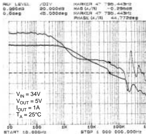
Full-Load Stability Phase Margin = 45 ^\circ
