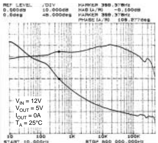
No-Load Stability Phase Margin = 109 ^\circ
