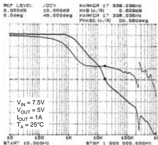
Full-Load Stability Phase Margin = 56 ^\circ
