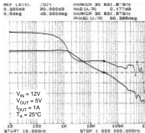
Full-Load Stability Phase Margin = 50 ^\circ
