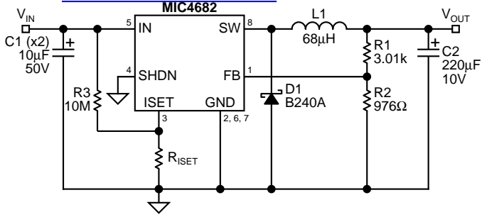
Current Limit Test Circuit
