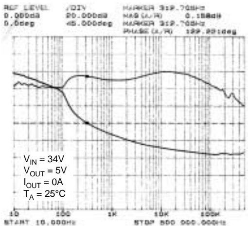
No-Load Stability Phase Margin = 122 ^\circ
