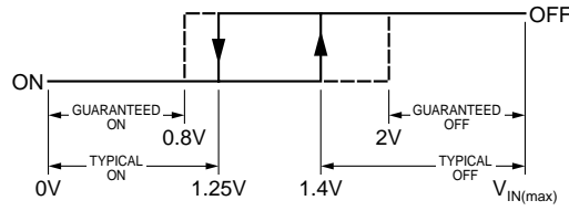
Shutdown Hysteresis
