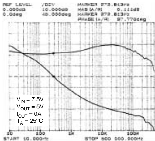
No-Load Stability Phase Margin = 98 ^\circ
