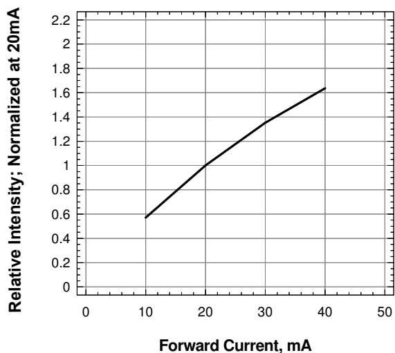
Relative Luminous Intensity Vs. Forward Current 查询 DDT DS-VW2-1 供应商
