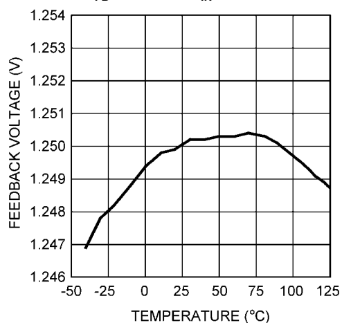
V_{FB} vs. Temp ( V_{IN} = 24V )
