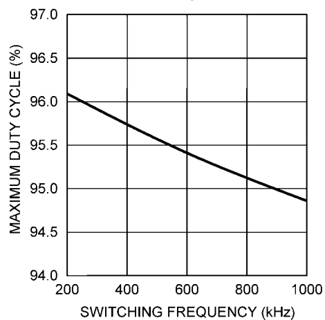
Max Duty Cycle vs. f_{SW} ( T_A = 25^\circ C )
