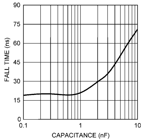
OUT Pin t_{FALL} vs. Gate Capacitance
