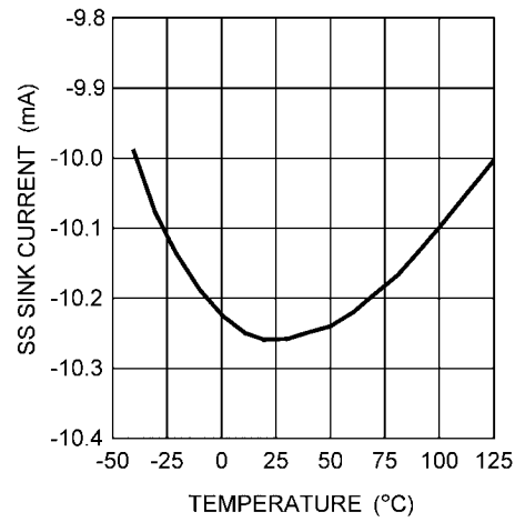
SS vs. Temperature
