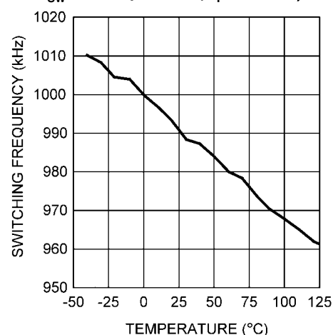
f_{SW} vs. Temperature ( R_T = 16.2 k\Omega )
