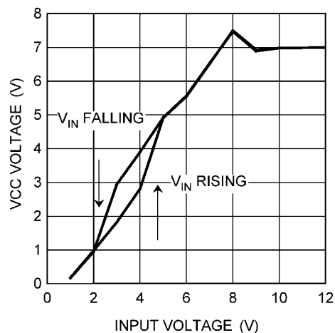
V_{CC} vs. V_{IN} ( T_A = 25^\circ C )
