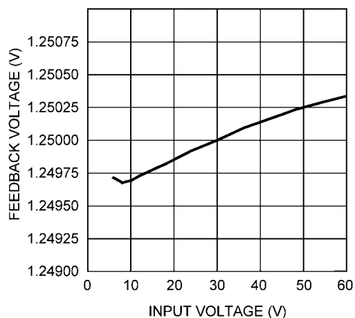
V_{FB} vs. V_{IN} ( T_A = 25^\circ C )
