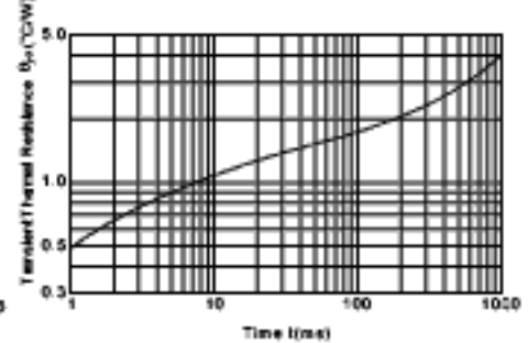
θ J-c -t Characteristics
