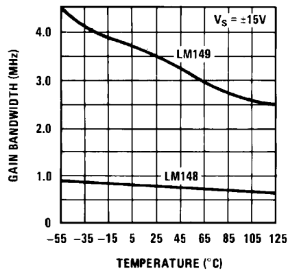
Gain Bandwidth
