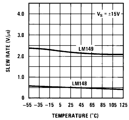
Slew Rate
