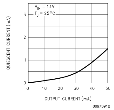
Quiescent Current
