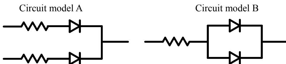
(A)Recommended circuit.
