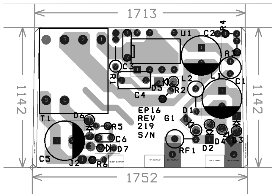
Figure 2 – PCB Layout
