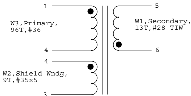
Figure 3 – Transformer Winding
