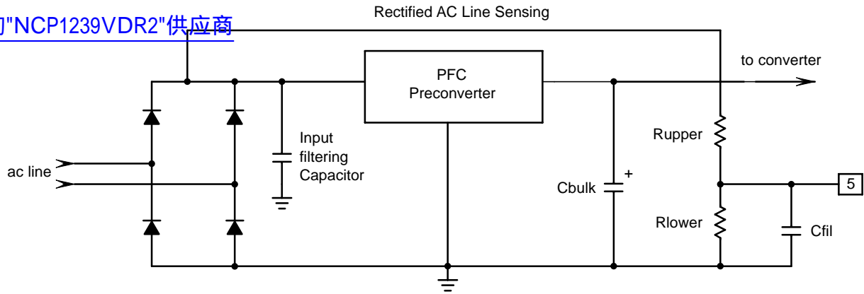
A second option to directly sense the mains
