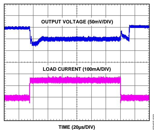
Figure 26. Load Transient Response, 0 mA to 150 mA ( V_{IN} = 3.6 V, Auto Mode)
