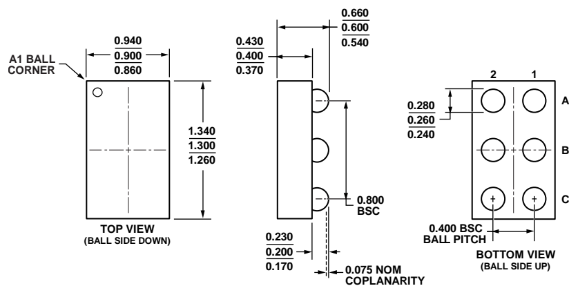
Figure 59. 6-Ball Wafer Level Chip Scale Package (WLCSP) (CB-6-4)
