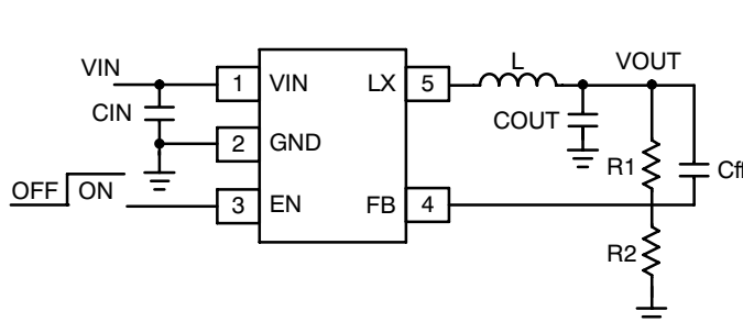
Figure 1. Typical Application - TSOP-5
