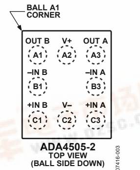
Figure 2. 8-Ball WLCSP (CB-8-2)
